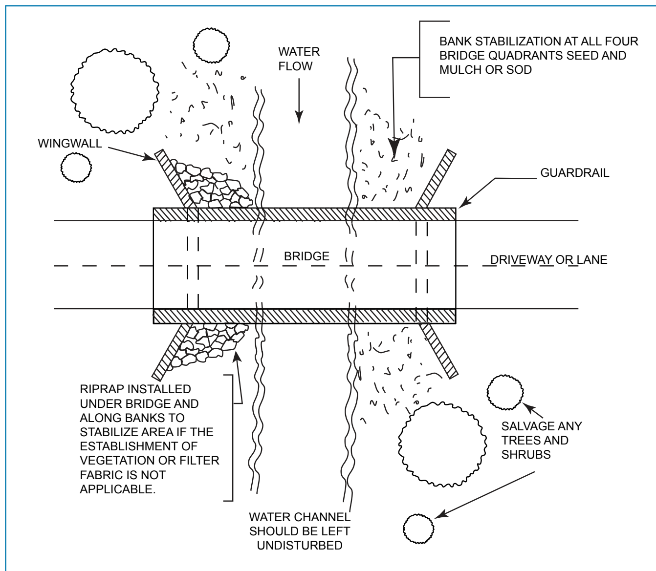
Figure 3.1-1. Plan view of bridge
